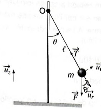
Figure 1 - Pendule simple
