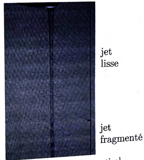
FIGURE 7 - Jet vertical
